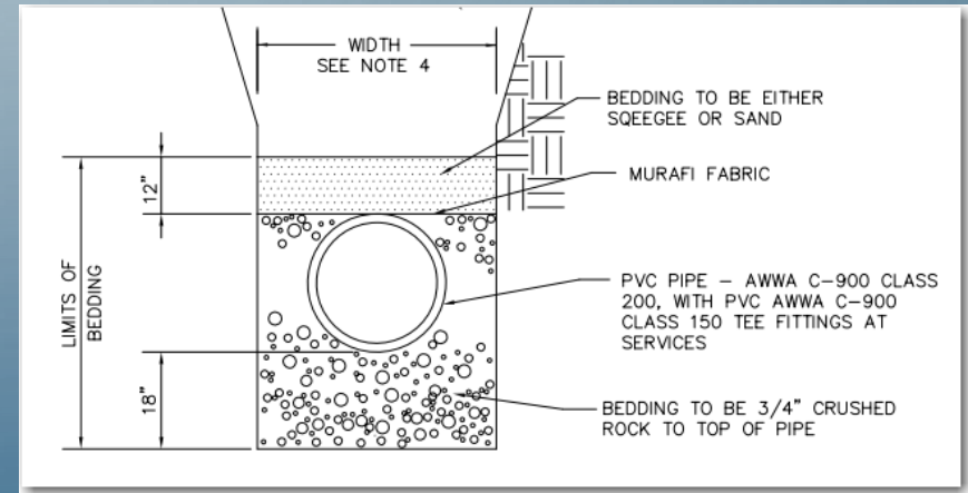
Expansive Soil Detail
